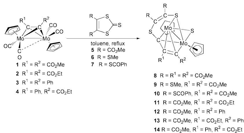
Scheme 2 Reactions of the dimolybdenum alkyne complexes with 1,3-dithiole-2-thiones.
