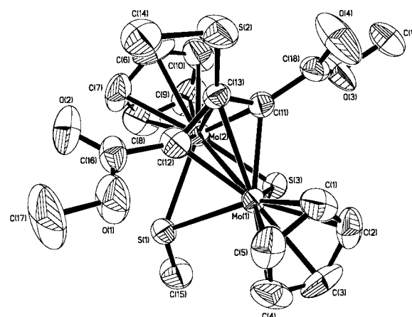
Fig. 4 Molecular structure of [\text{Mo}_2(\mu\text{-S})\{\mu\text{-SMe}\}\{\mu\text{-C}(\text{CO}_2\text{Me})\text{-C}(\text{SMe})=\text{C}(\text{CO}_2\text{Me})\}\text{Cp}_2] 17 . Only molecule 1 of the two independent molecules in the unit cell is shown.
