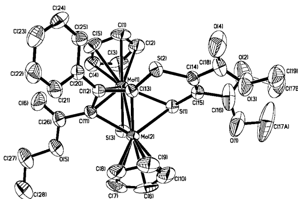
Fig. 3 Molecular structure of [\text{Mo}_2(\mu\text{-S})\{\mu\text{-SC}(\text{CO}_2\text{Me})=\text{C}(\text{CO}_2\text{Me})\text{-SCC}(\text{Ph})=\text{C}(\text{CO}_2\text{Et})\}; \text{Cp}_2] 14 .
