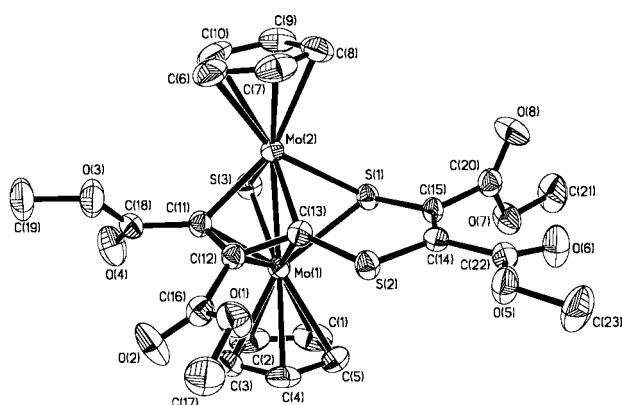
Fig. 1 Molecular structure of [Mo 2 (μ-S){μ-SC(CO 2 Me)=C(CO 2 Me)-SCC(CO 2 Me)=C(CO 2 Me)}Cp 2 ] 8 in the crystal showing the atomic numbering scheme.
