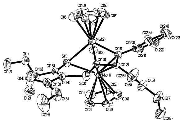
Fig. 2 Molecular structure of [\text{Mo}_2(\mu\text{-S})\{\mu\text{-SC}(\text{CO}_2\text{Me})=\text{C}(\text{CO}_2\text{Me})\text{-SCC}(\text{CO}_2\text{Et})=\text{C}(\text{Ph})\}; \text{Cp}_2] 13 .
