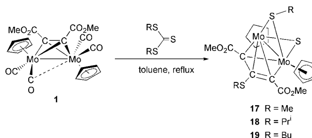
Scheme 4 Reactions of complex 1 with acyclic trithiocarbonates.
